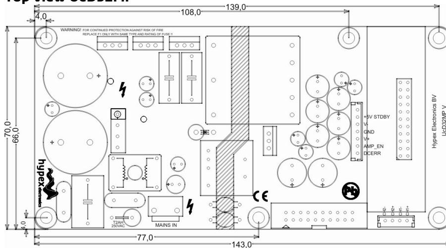
Top view UcD32MP
