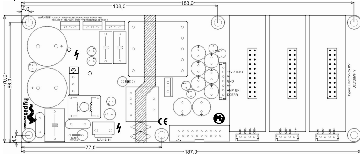
Top view UcD34MP
